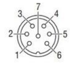
Front side molded 7P Male connector
